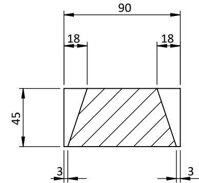
SECTION A-A Leg Notch Cut Out Profile
